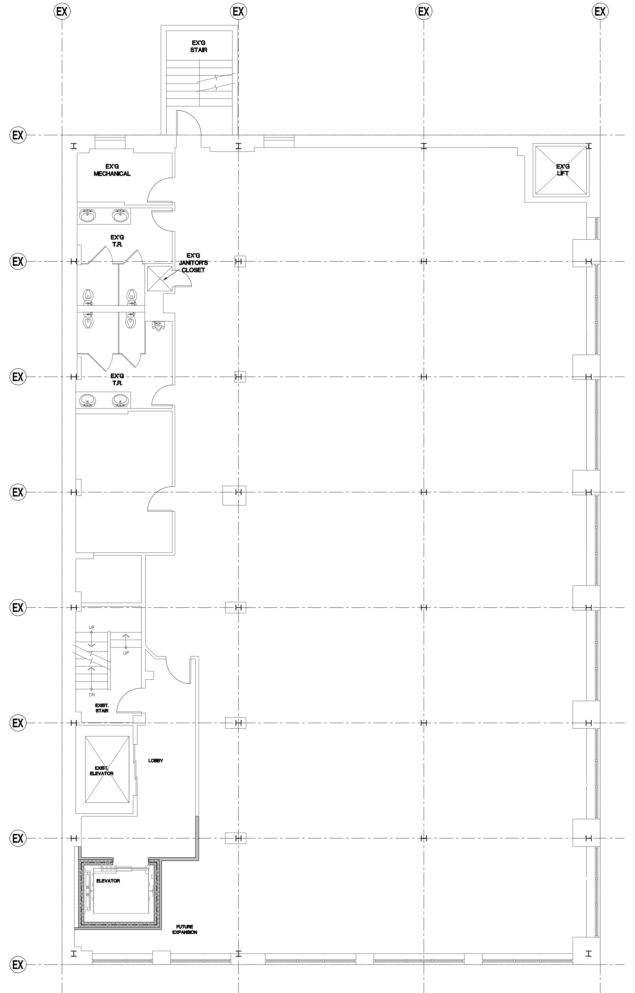
4th FLOOR PROPOSED PLAN SCALE: 1/4" = 1'-0"
